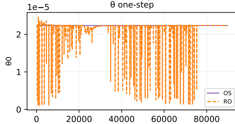
Oracle theta fit — sample 382
