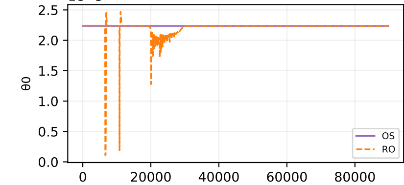
Oracle theta fit — sample 574
