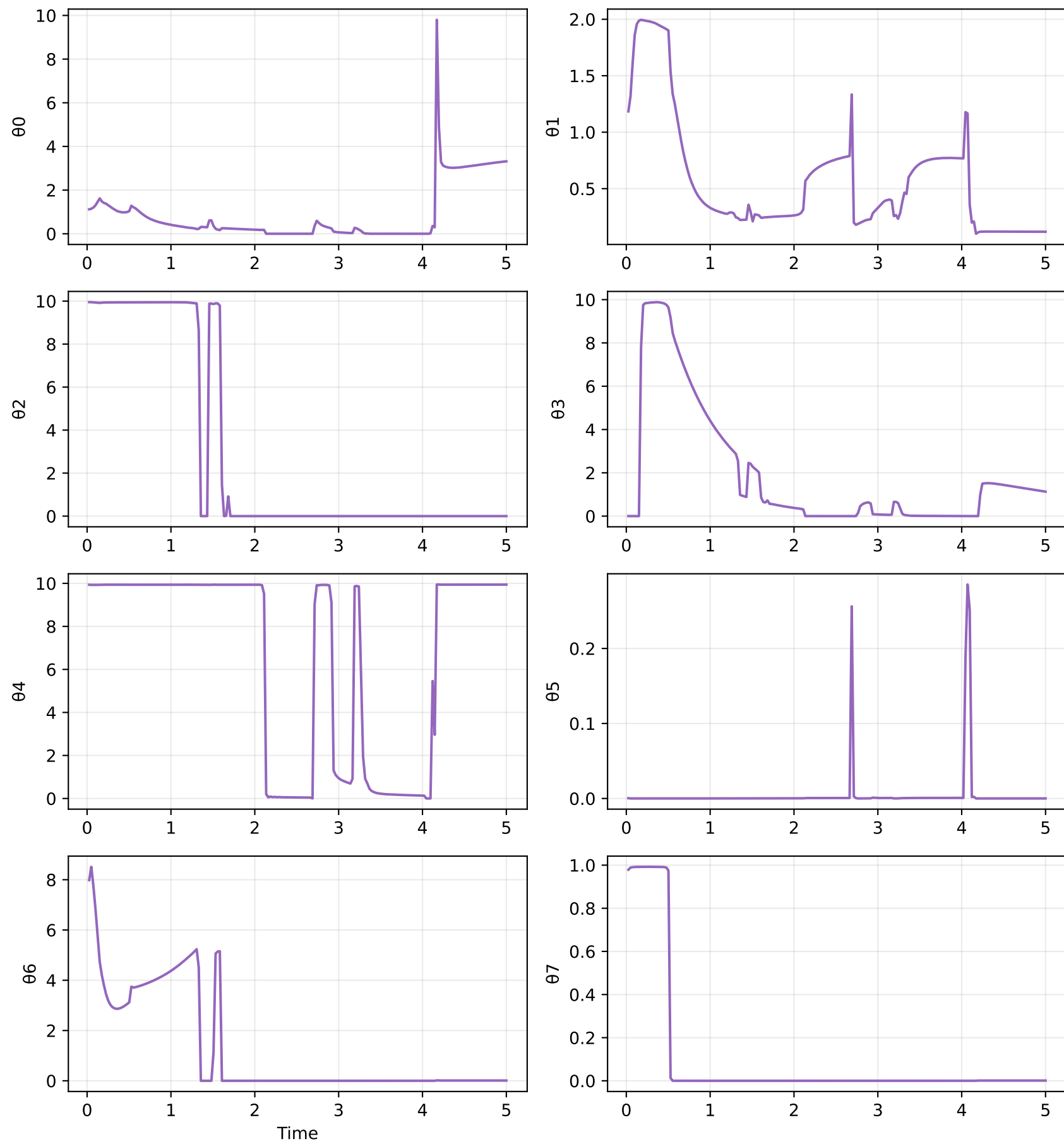
Oracle theta trajectories (rollout) — methane_revWGS_ohgate_no (P=7) sample 0
