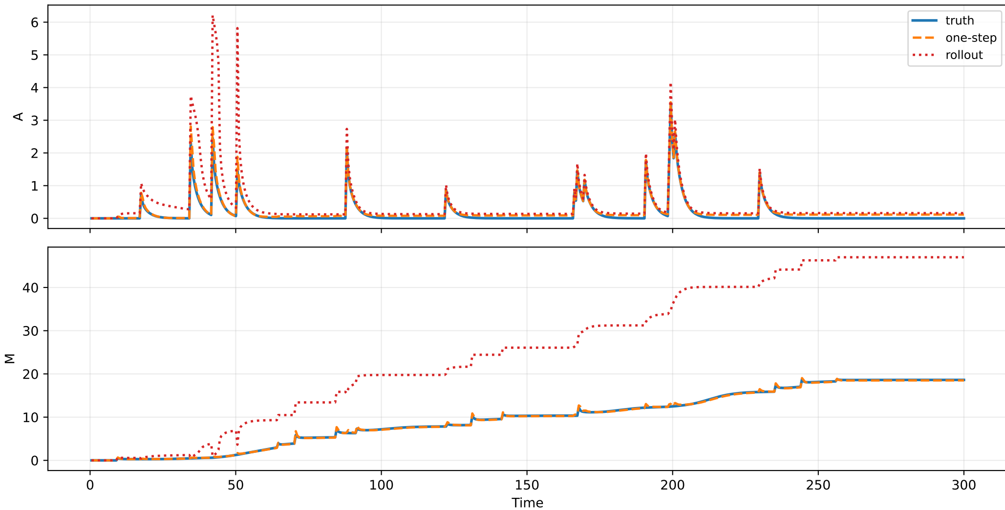
Oracle per-step fit — reduced2 (sample 1)
