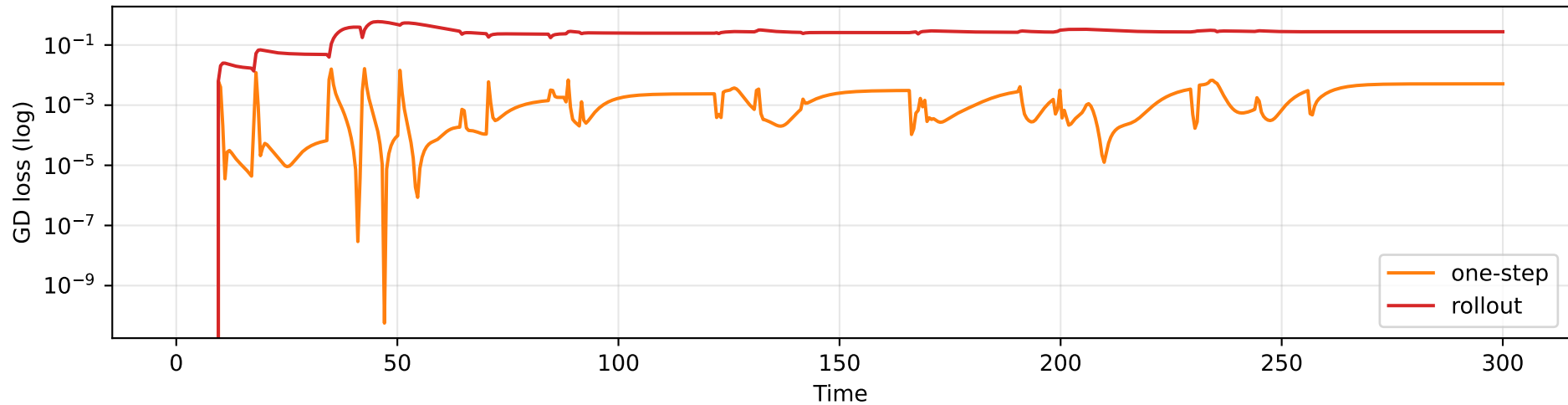
Per-step GD loss at convergence — reduced3
