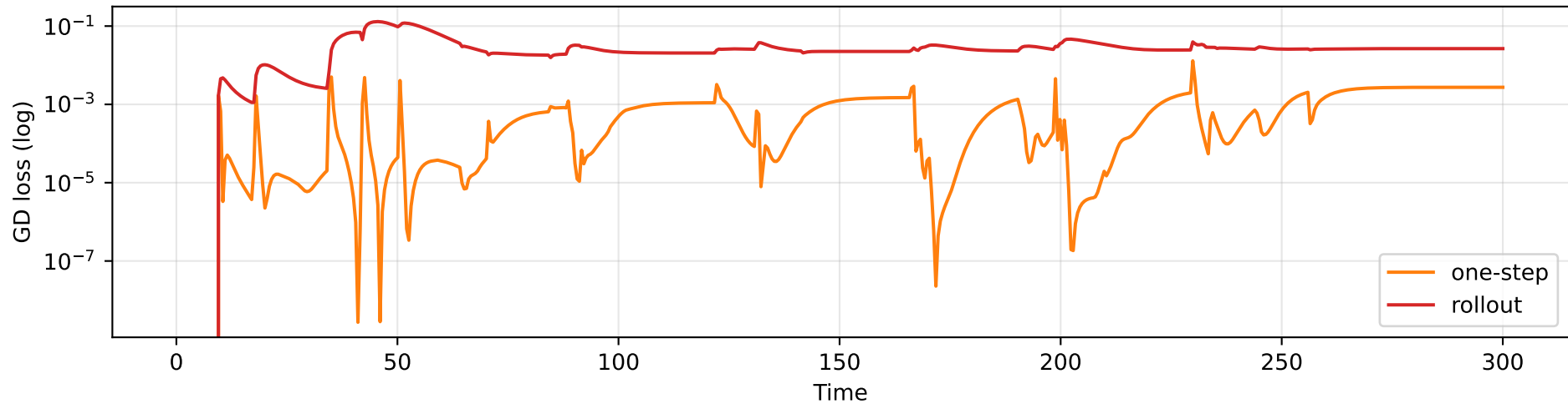
Per-step GD loss at convergence — reduced6_ADGJLM
