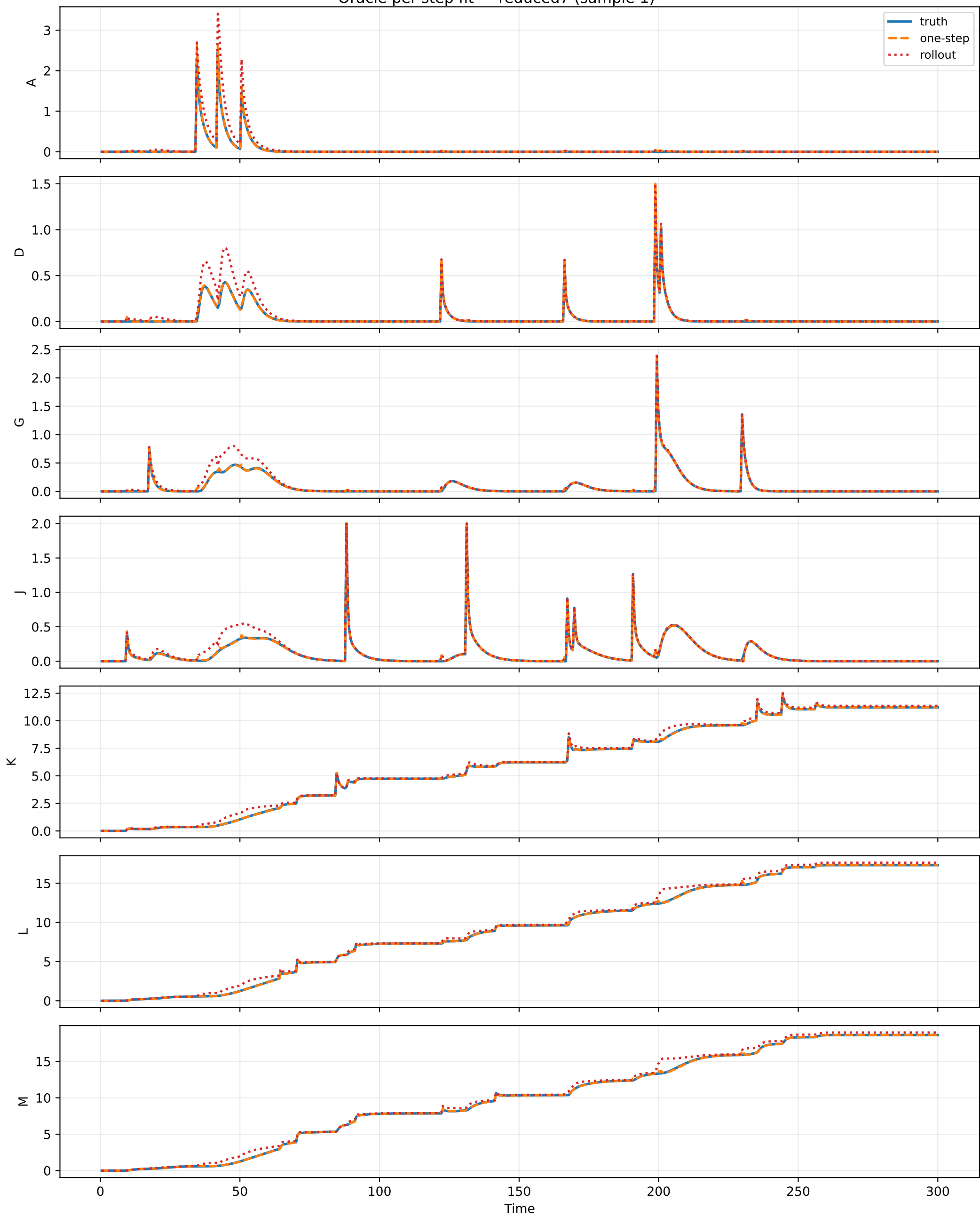
Oracle per-step fit — reduced7 (sample 1)
