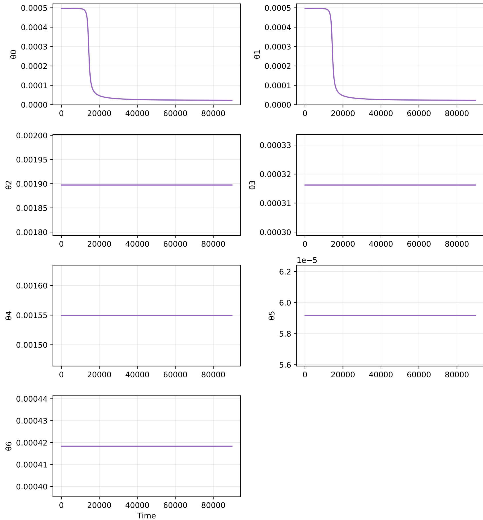
Oracle theta trajectories (rollout) — txtl_resource_and_maturation_dna (P=7) sample 427
