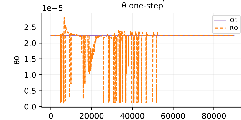
Oracle theta fit — sample 17
