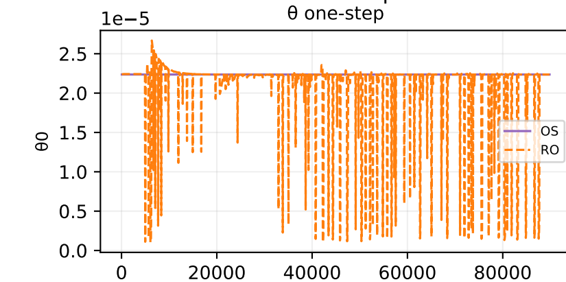
Oracle theta fit — sample 21
