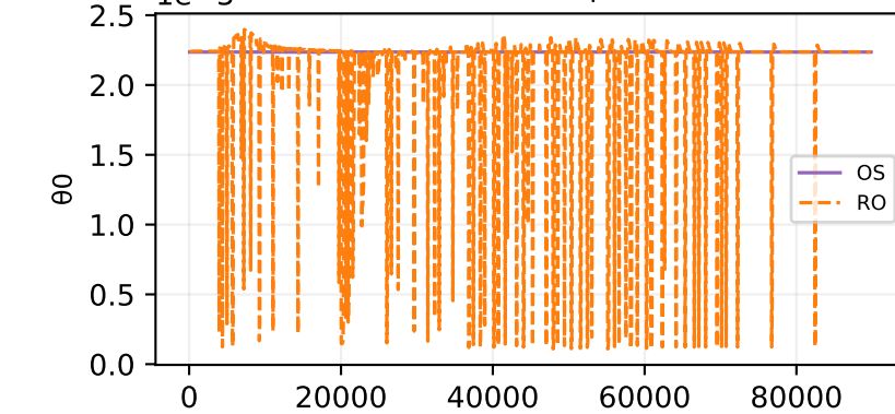
Oracle theta fit — sample 43
