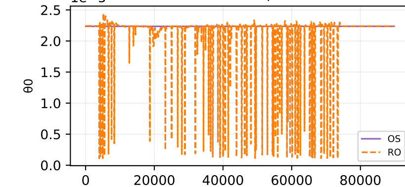
Oracle theta fit — sample 69
