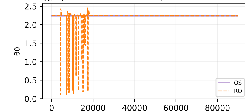
Oracle theta fit — sample 97
