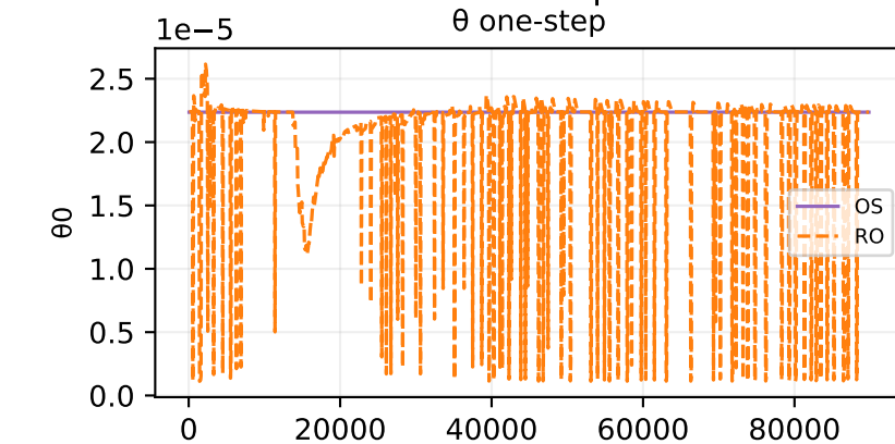
Oracle theta fit — sample 130
