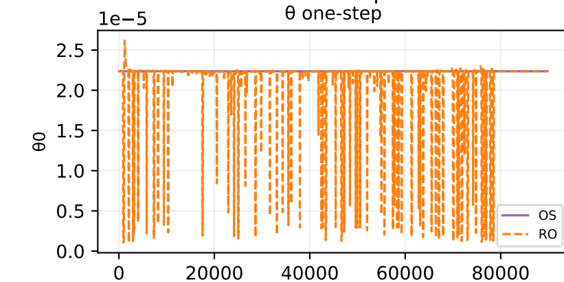
Oracle theta fit — sample 144
