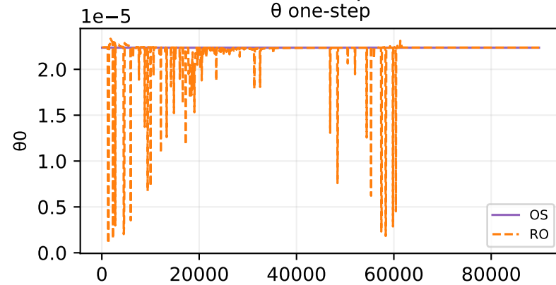
Oracle theta fit — sample 332
