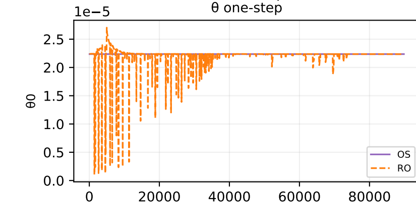
Oracle theta fit — sample 450
