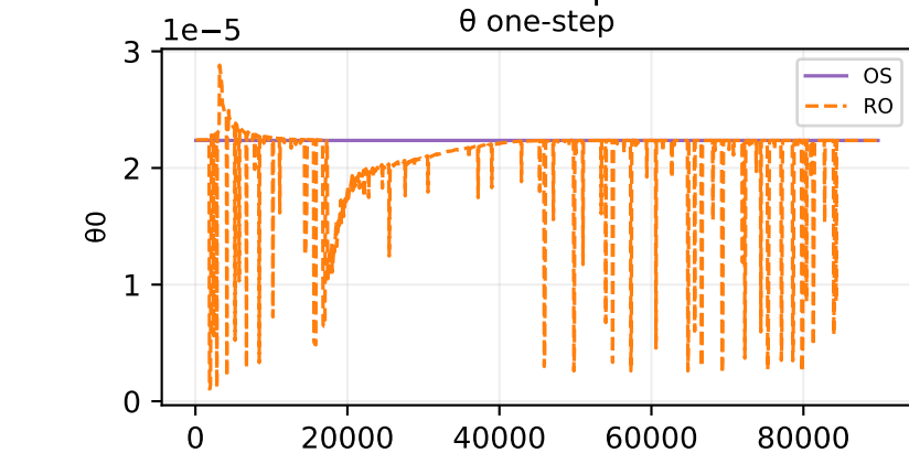
Oracle theta fit — sample 486
