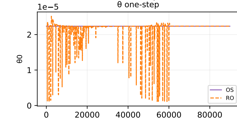
Oracle theta fit — sample 513
