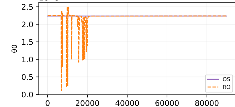
Oracle theta fit — sample 588 θ one-step
