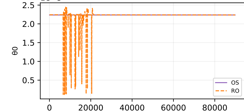
Oracle theta fit — sample 636 \theta one-step
