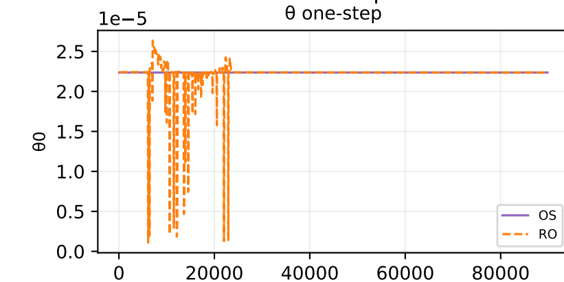
Oracle theta fit — sample 648
