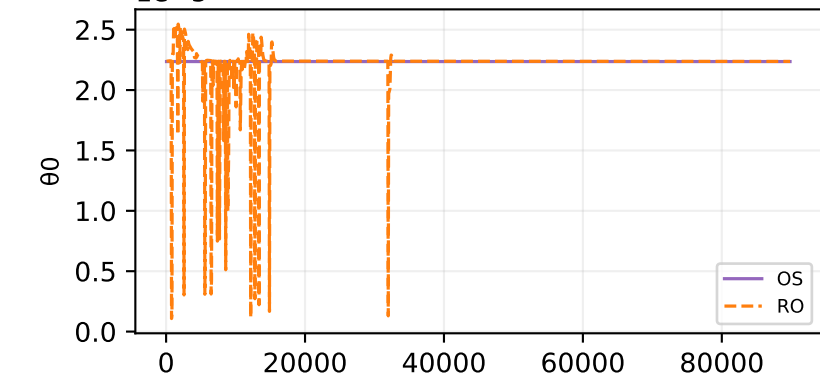
Oracle theta fit — sample 672 \theta one-step
