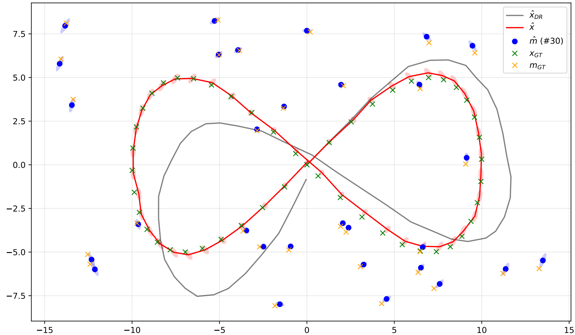
SLAM result at step 49 (with marginals)
