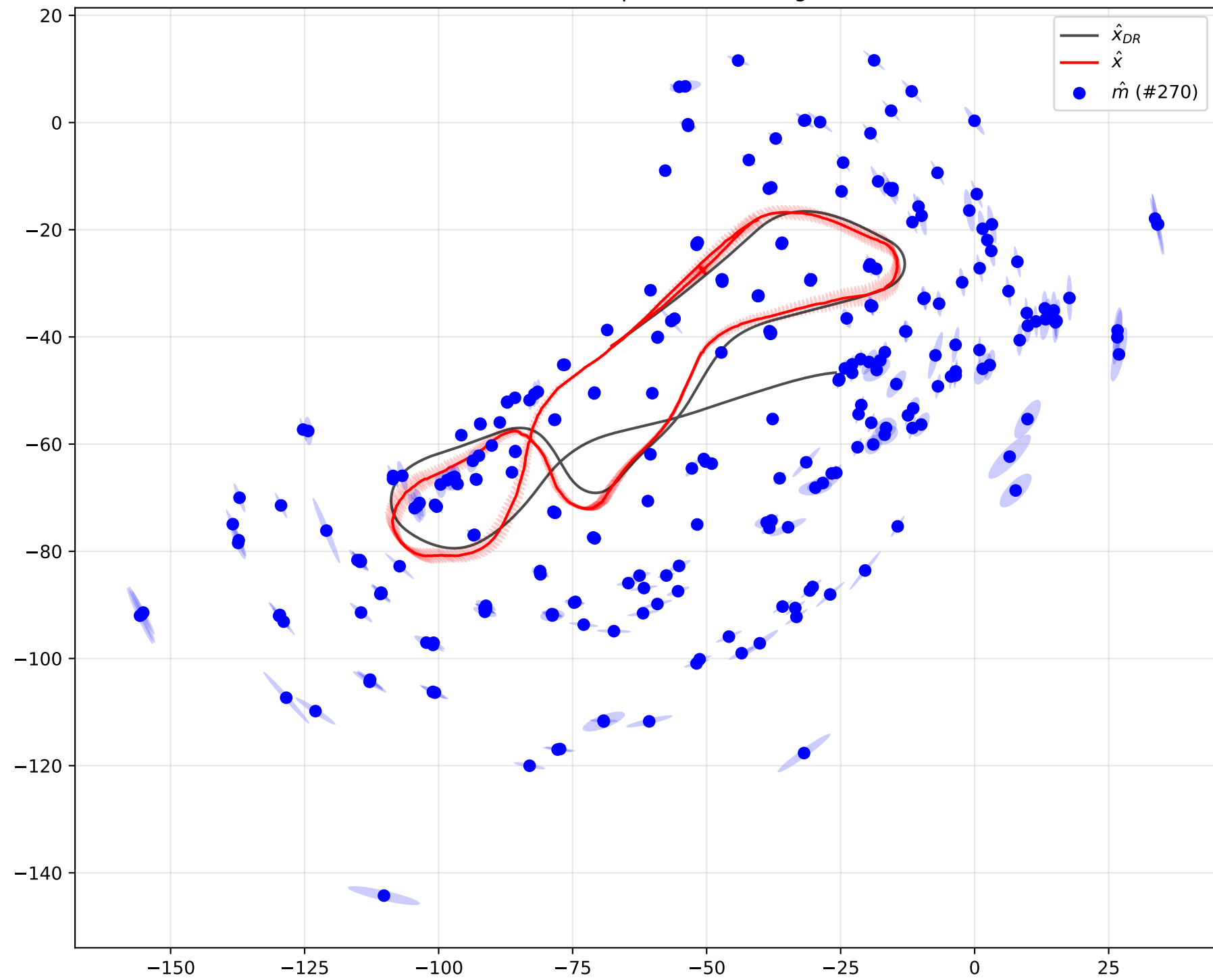
SLAM result at step 585 (with marginals)
