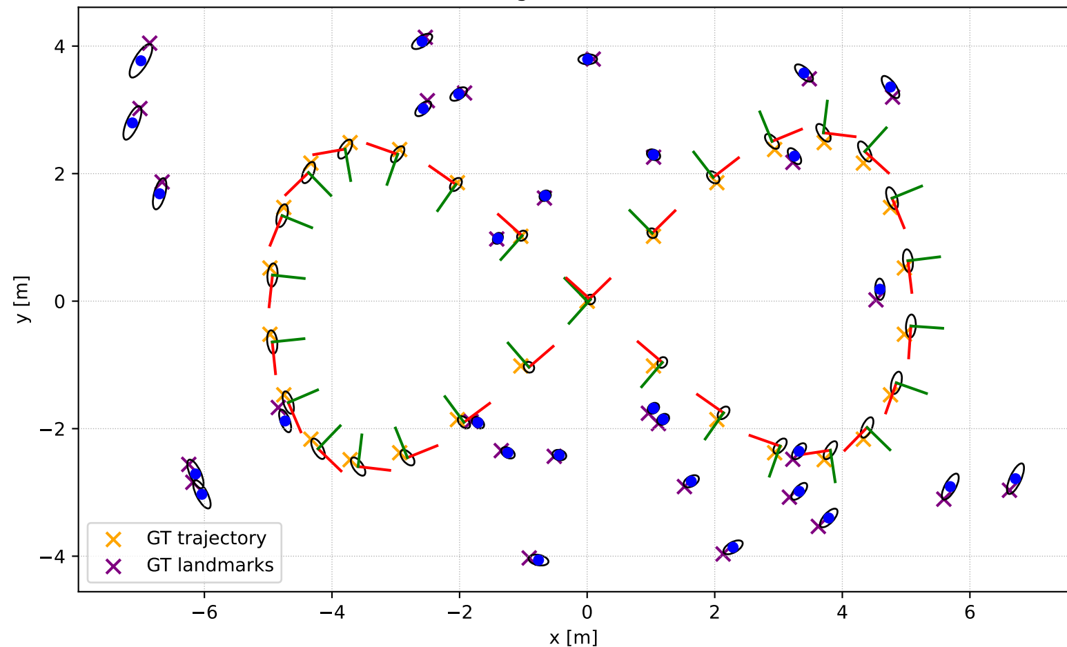
Nonlinear 2D SLAM: SLAM with ground truth associations vs Ground Truth
