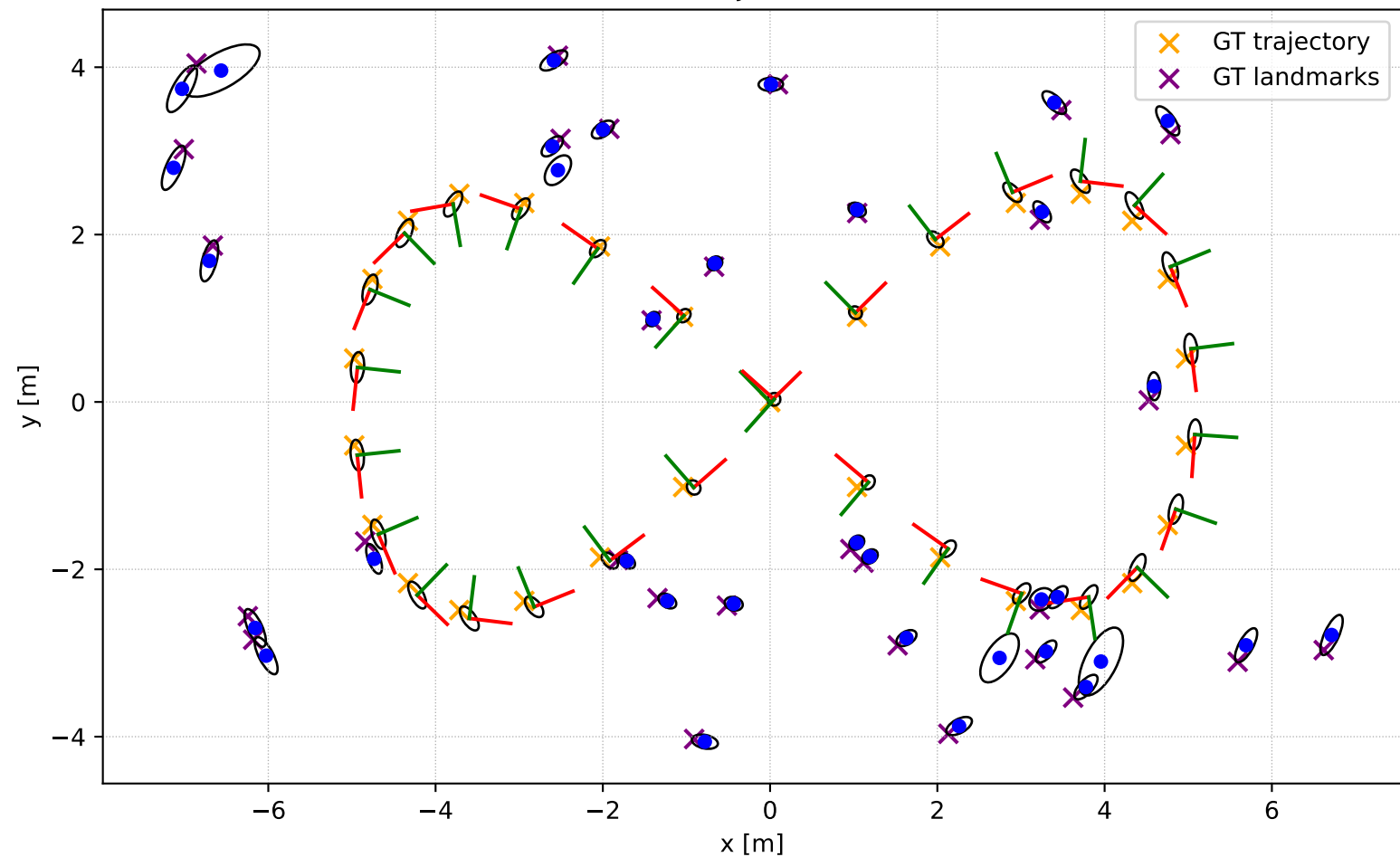
Nonlinear 2D SLAM: SLAM with jccb associations vs Ground Truth
