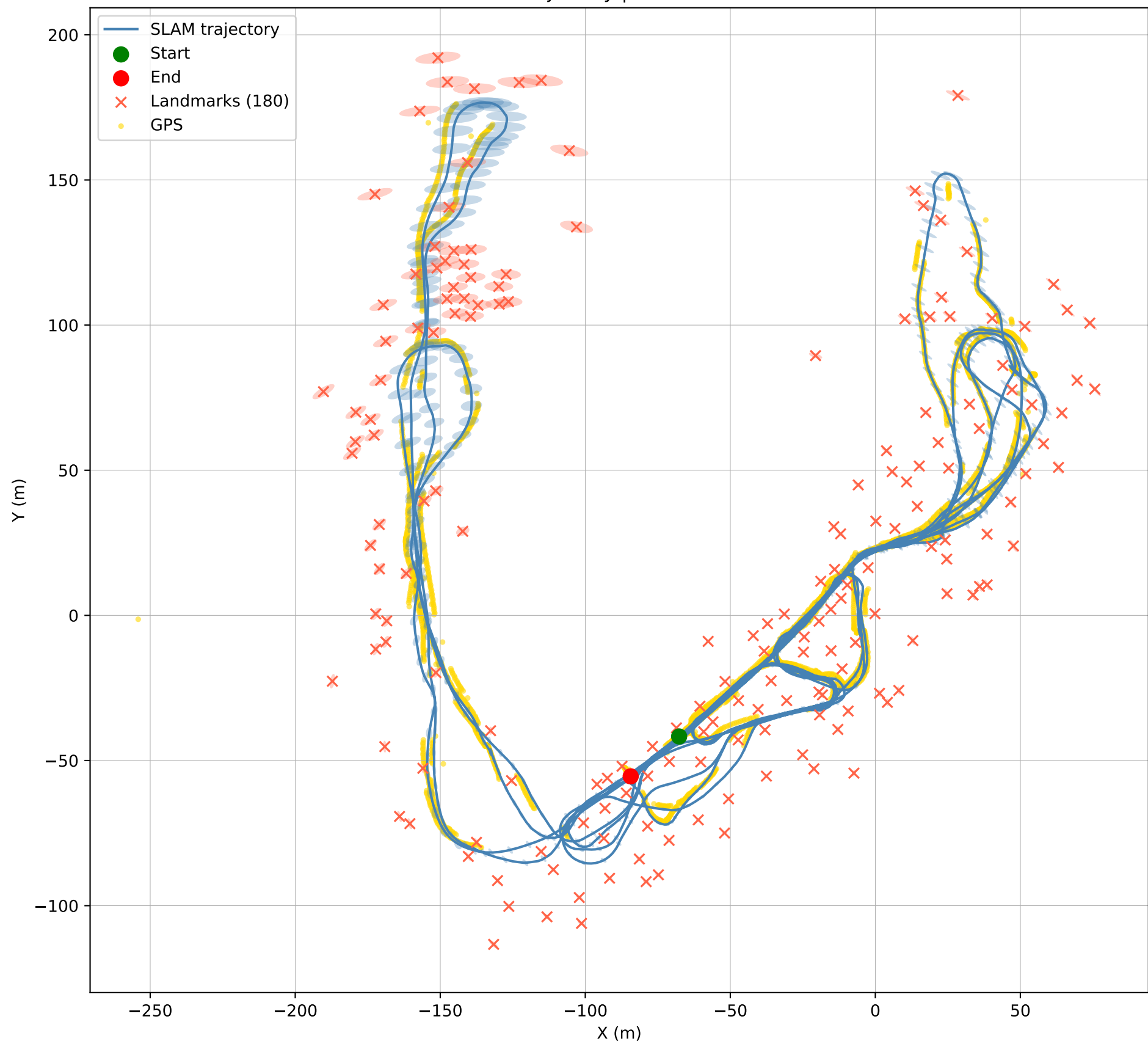
SLAM Trajectory | 180 landmarks
