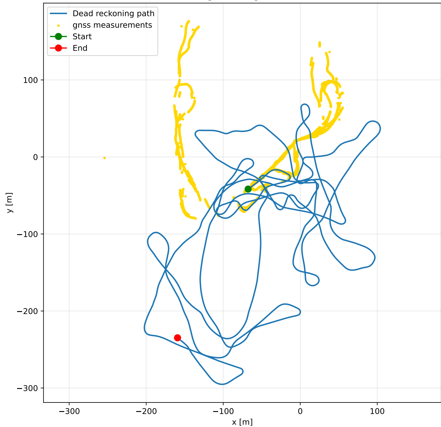
Dead Reckoning Path vs gnss Measurements
