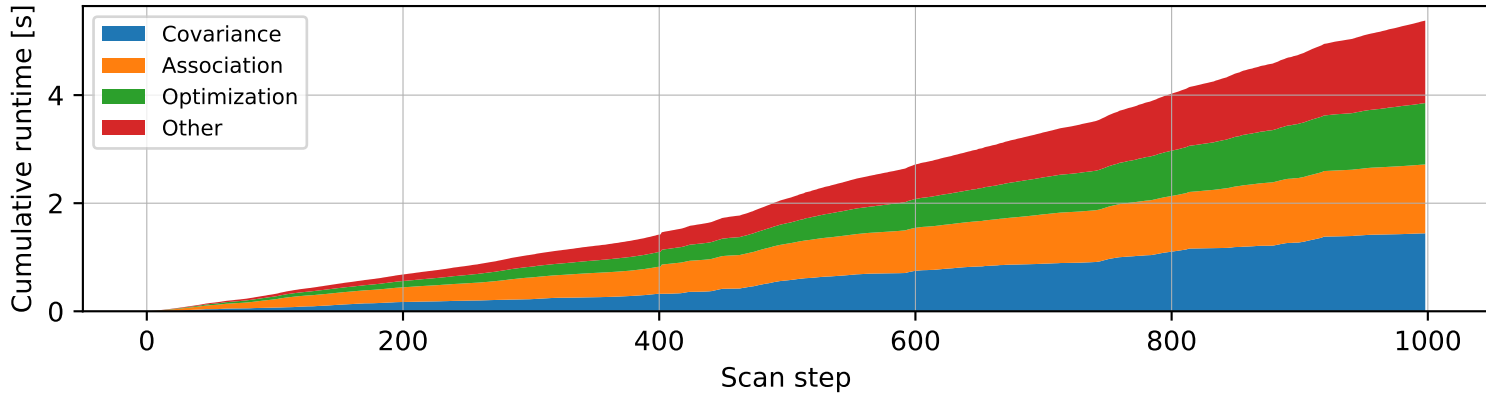
Cumulative Runtime by Component (median total: 5.38 s)
