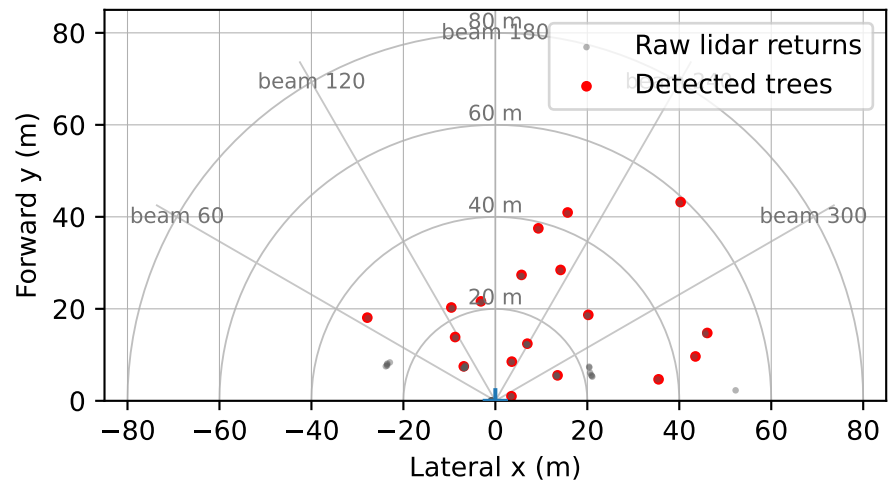
Scan 2416 in sensor frame
