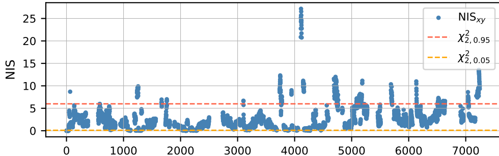
Position NIS (ANIS = 2.49)
