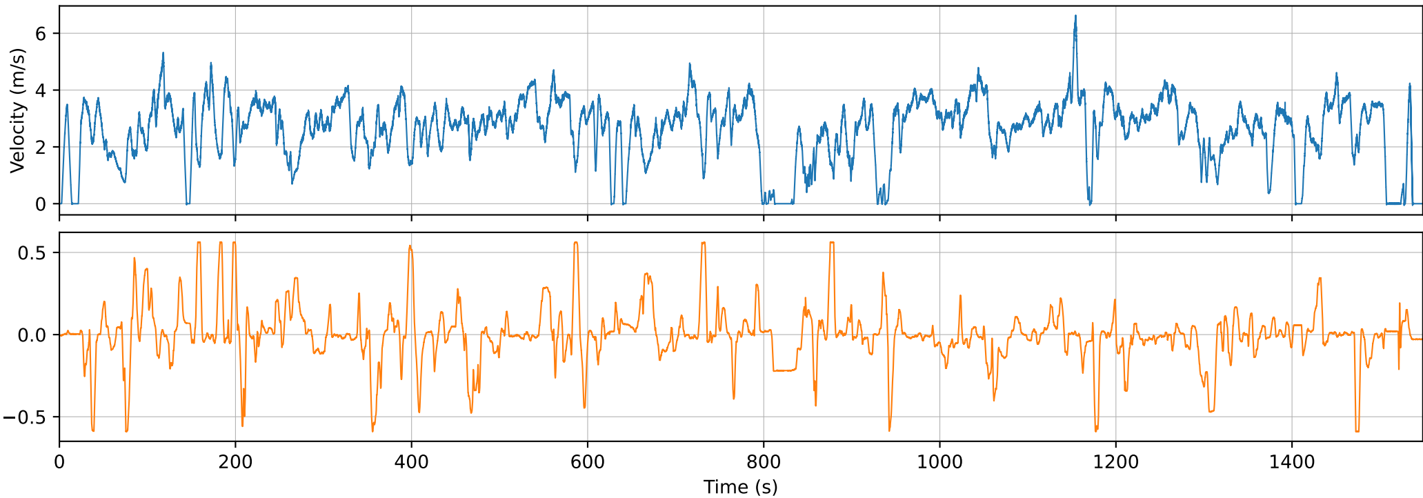
Raw odometry measurements
