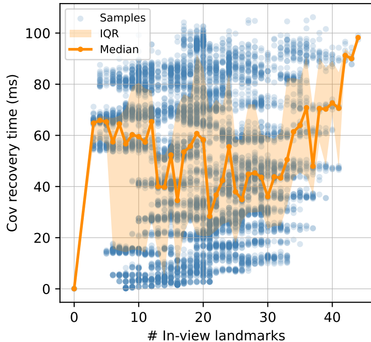
Spearman rho: \rho = 0.04
