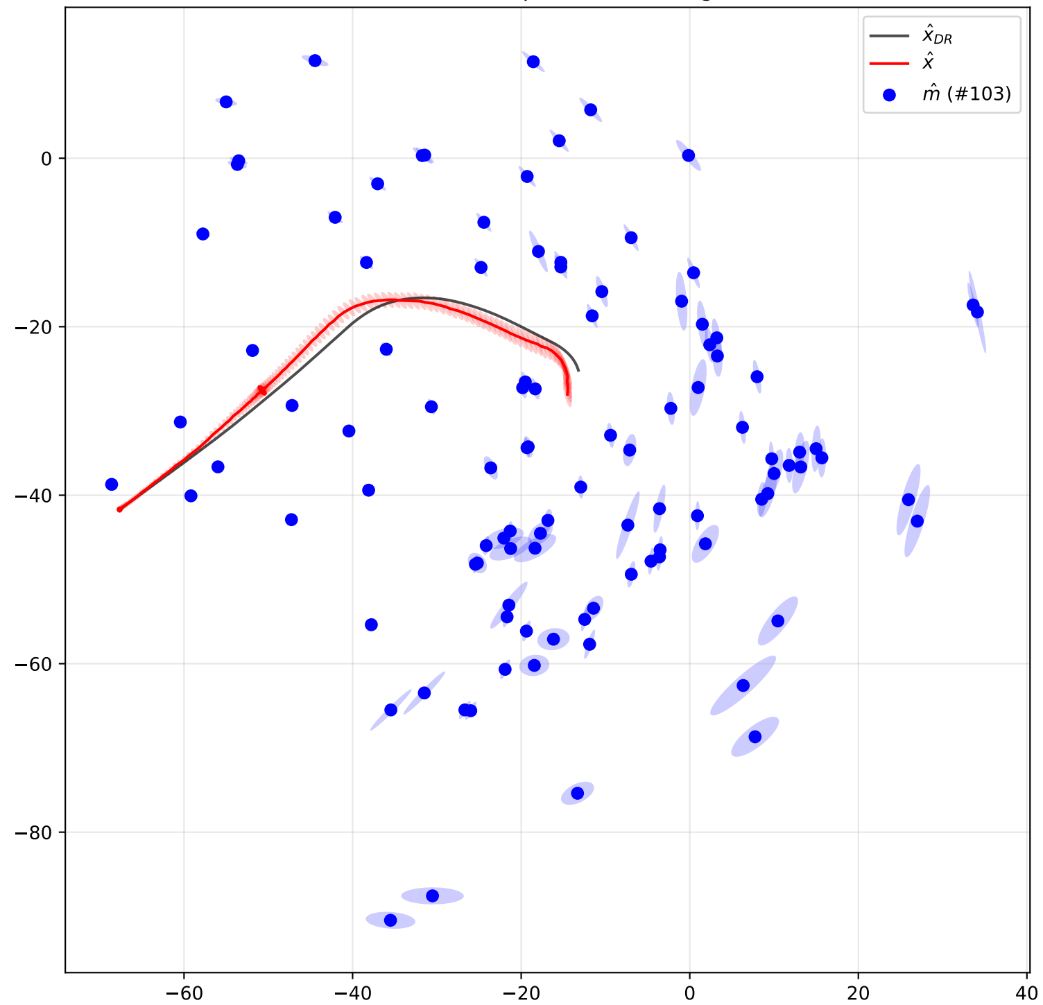
SLAM result at step 176 (with marginals)
