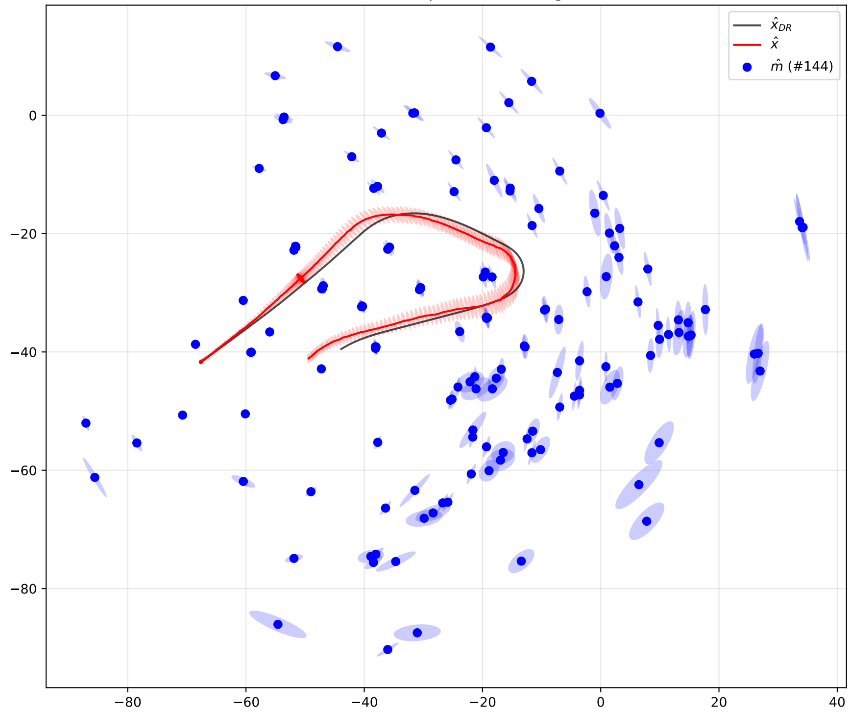
SLAM result at step 234 (with marginals)
