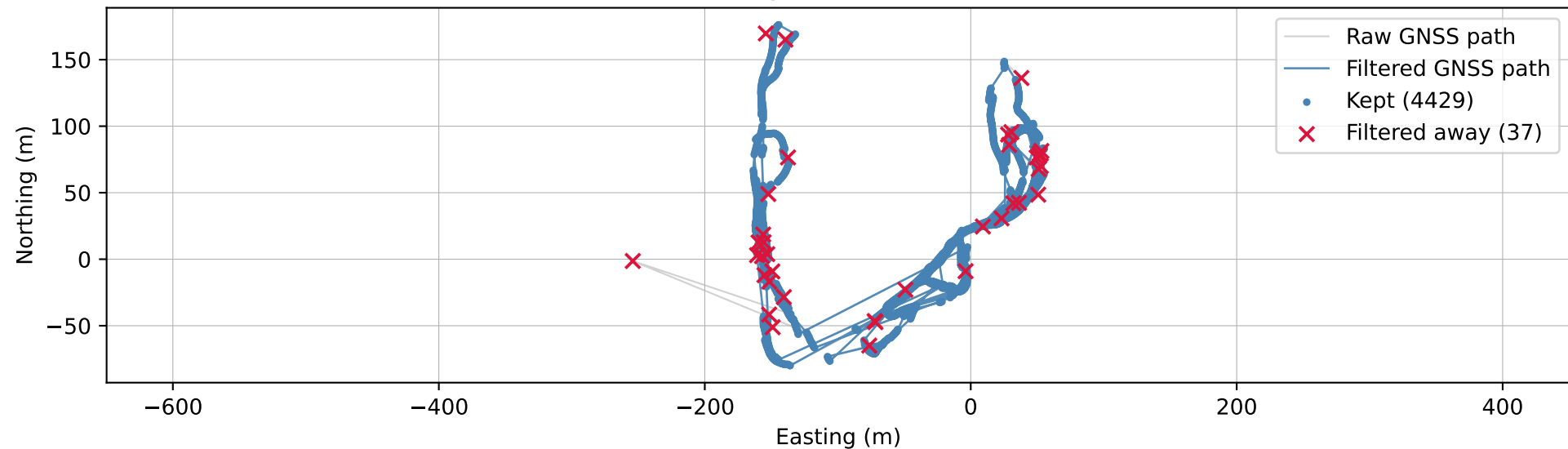
GNSS filtering in Victoria Park loader
