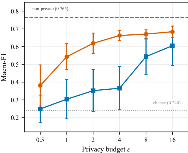
(a) Utility
