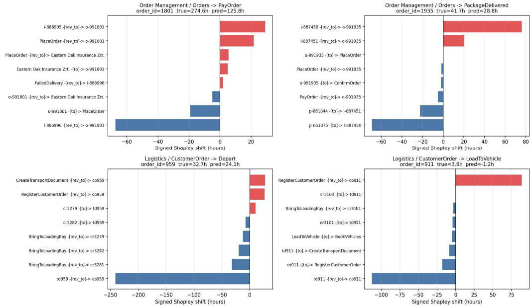
Figure 5.11: Graphs showing the single-trace explanations generated indicating the most important edges in each trace as well as the impact on the model's prediction.
