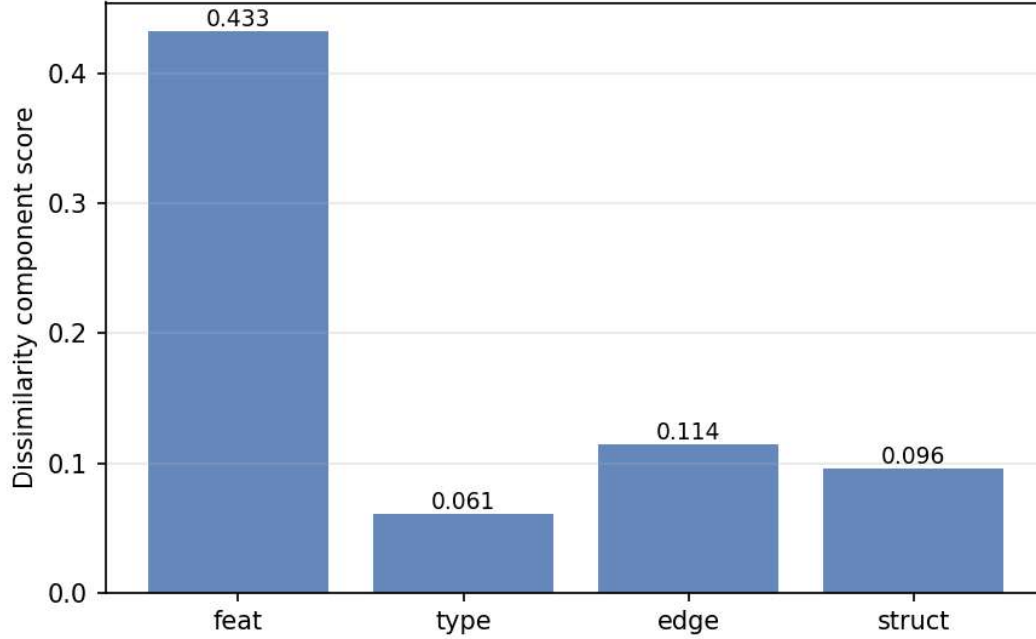
Figure 5.21: Graph representation of the dissimilarity values for the distinct elements compared between the user's chosen graph and the chosen counterfactual.
