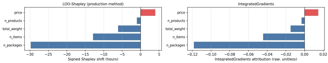
Figure 5.16: Graphs showing the single-trace explanation provided for feature importance on the Order node using the Integrated Gradients method for identification and the LOO-Shapley method for quantifying the feature's impact on the prediction.
