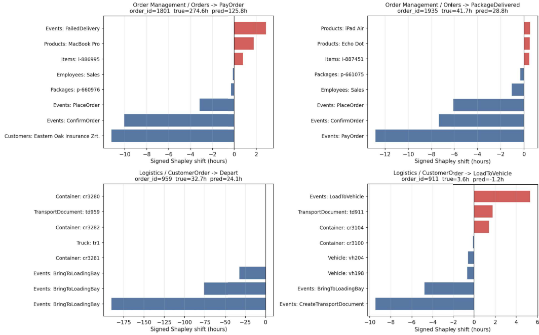
Figure 5.10: Graphs showing the single-trace explanations generated indicating the most important nodes in each trace as well as the impact on the model's prediction.
