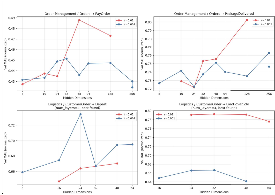
Figure 5.1: Normalized Val MAE scores for the HTG model per hyperparameter setting. Note: scales (y-axis) are not aligned, as I intended to compare hyperparameter settings within each KPI.
