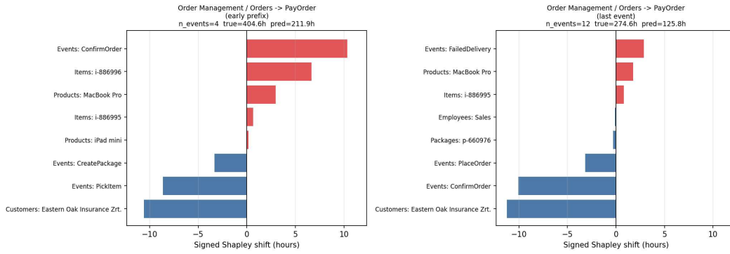
Figure 5.13: Graphs showing the single-trace explanations of node importance generated for two different prefixes of the same process execution.
