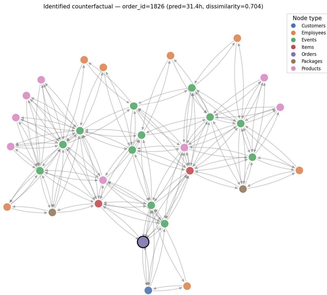
Figure 5.20: Graph representation of the counterfactual graph identified for counterfactual explanation.
