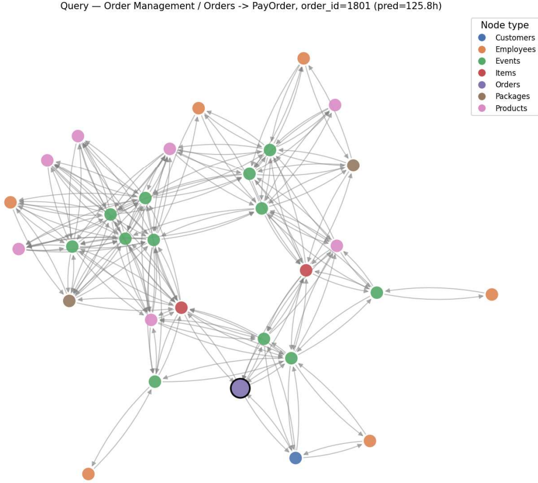
Figure 5.19: Graph representation of the user's selected graph for counterfactual explanation.
