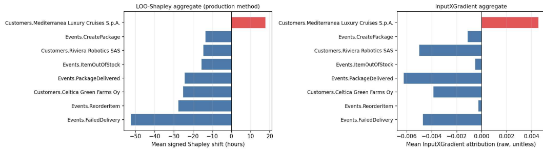
Figure 5.17: Graphs showing the aggregate explanation provided for feature importance of the nodes in the chosen traces using the Gradients · Input method for identification and the LOO-Shapley method for quantifying the feature's impact on the prediction.
