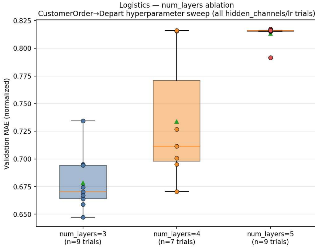
Figure 5.2: Normalized Val MAE scores for the HGT model on the Logistics dataset for KPI "Elapsed time from CustomerOrder to Depart" per different number of layers
