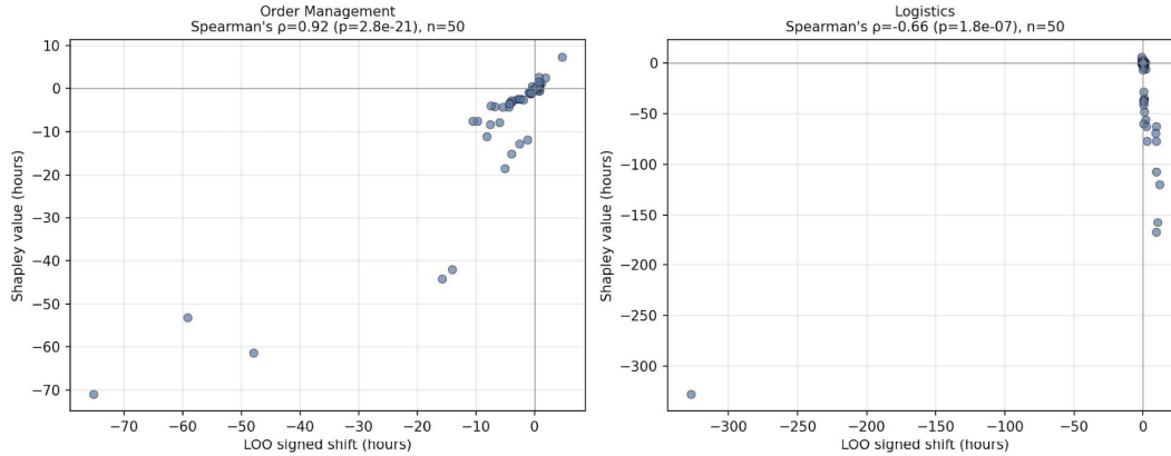
Figure 5.9: Measure of agreement between LOO method and full Shapley Values
