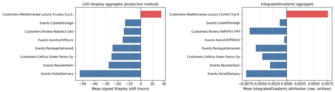
Figure 5.18: Graphs showing the aggregate explanation provided for feature importance of the nodes in the chosen traces using the Integrated Gradients method for identification and the LOO-Shapley method for quantifying the feature's impact on the prediction.
