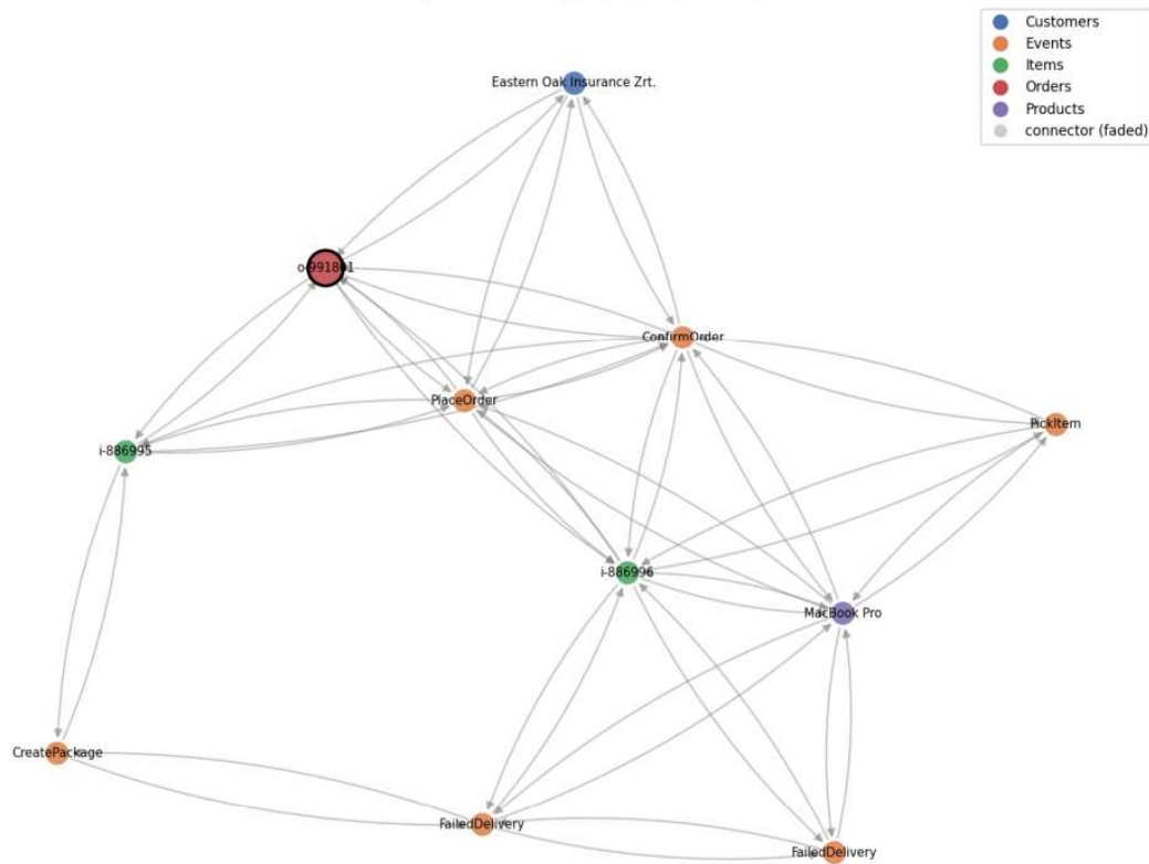
Figure 5.12: Example of a subgraph created using the identified most important nodes and edges for one of the traces shown before.
