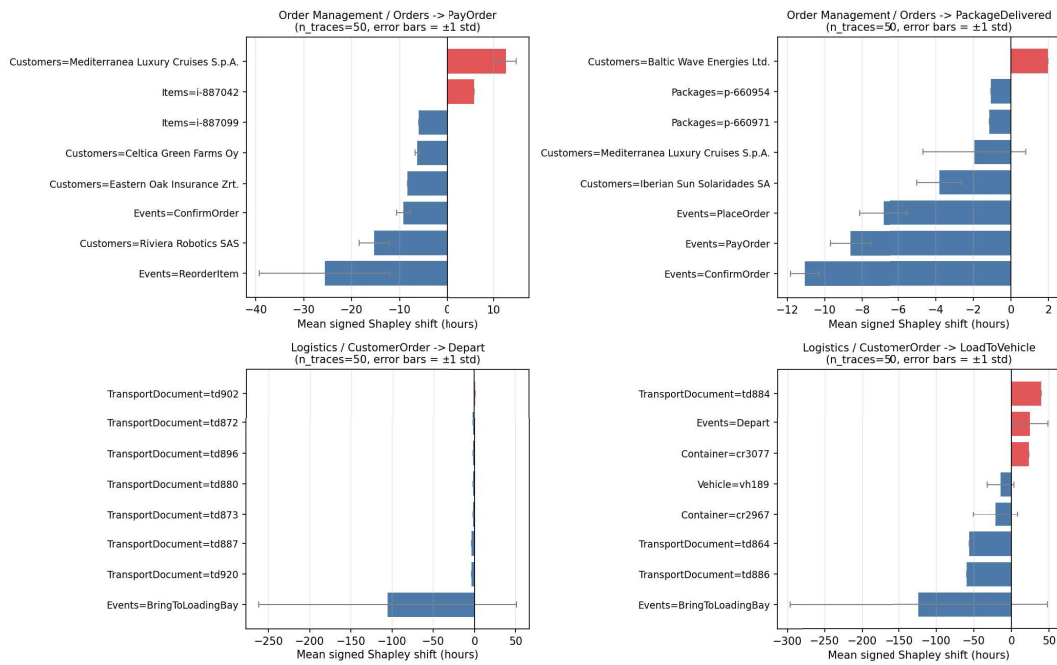
Figure 5.14: Graphs showing the aggregate explanations generated indicating the most important nodes for a collection of 50 traces as well as the impact on the model's prediction.
