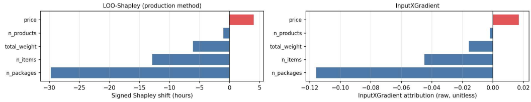
Figure 5.15: Graphs showing the single-trace explanation provided for feature importance on the Order node using the Gradient · Input method for identification and the LOO-Shapley method for quantifying the feature's impact on the prediction.
