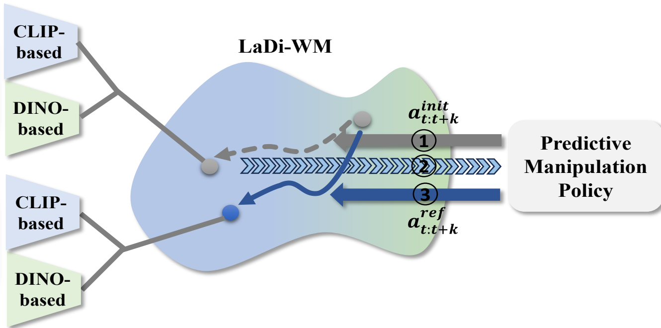
(a) Predictive policy refinement
