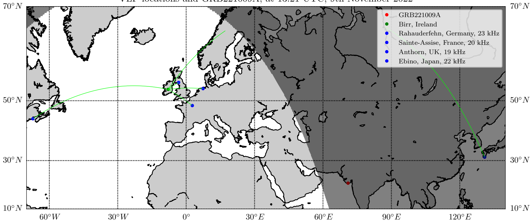
VLF locations and GRB221009A, at 13:21 UTC, 9th November 2022
