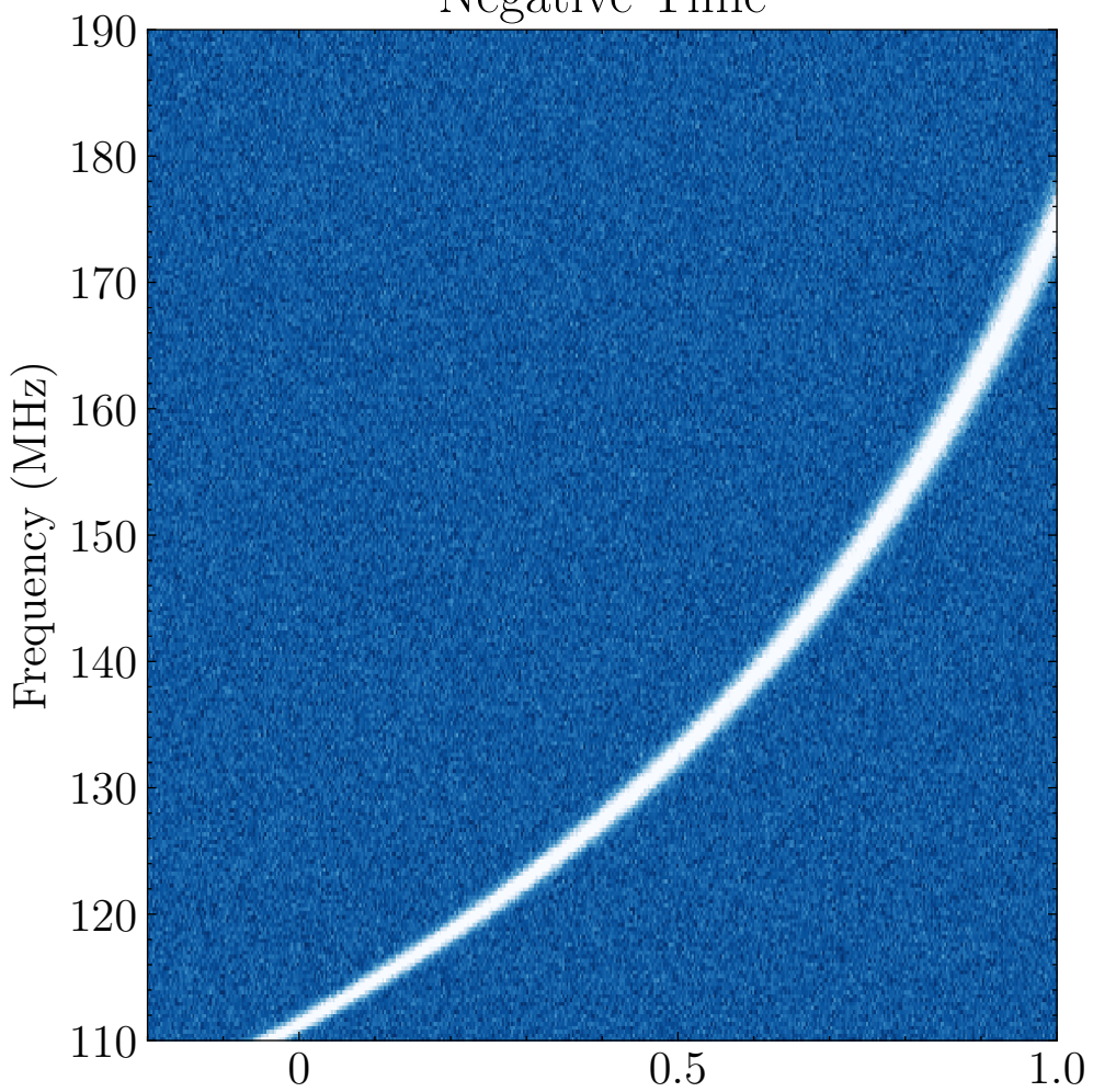
Negative Time
