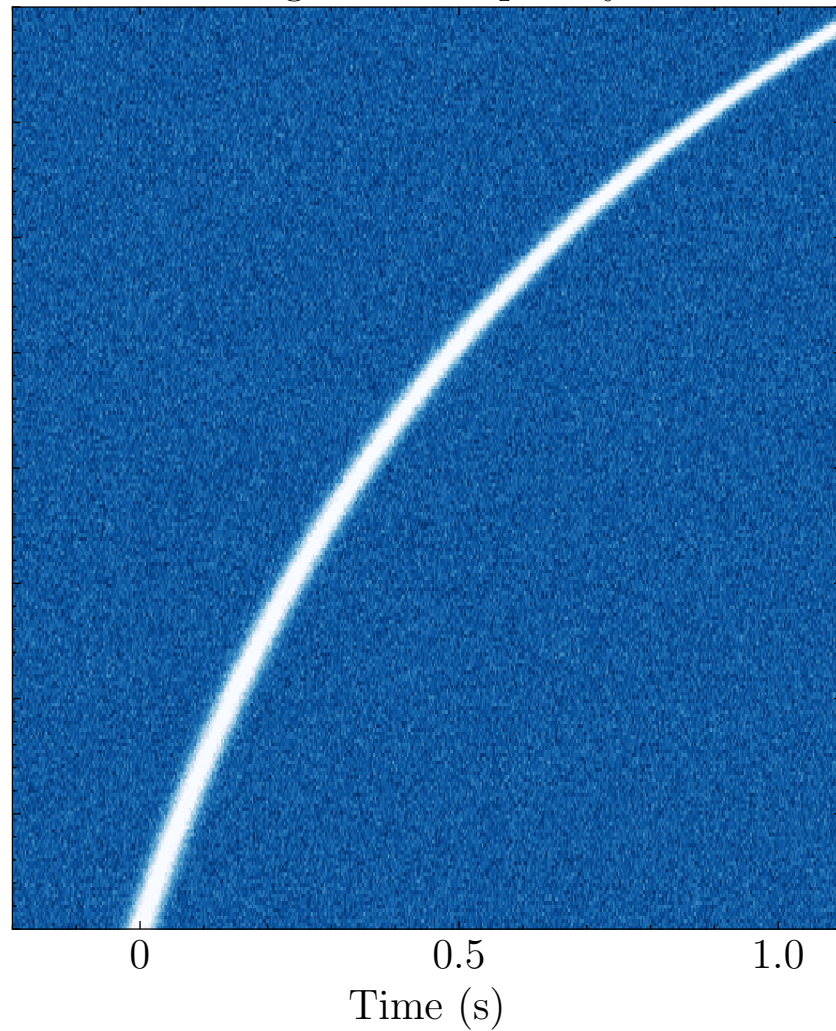
Negative Frequency
