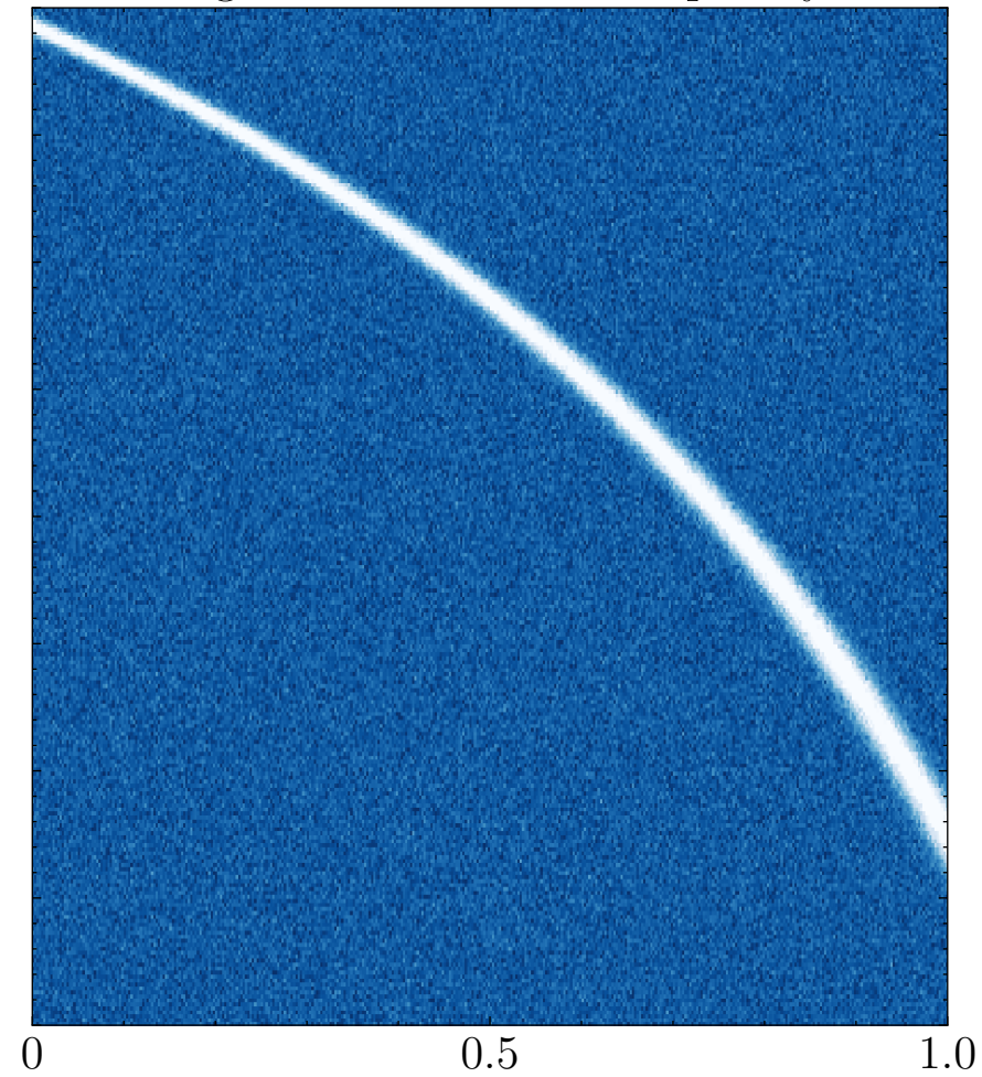
Negative Time and Frequency
