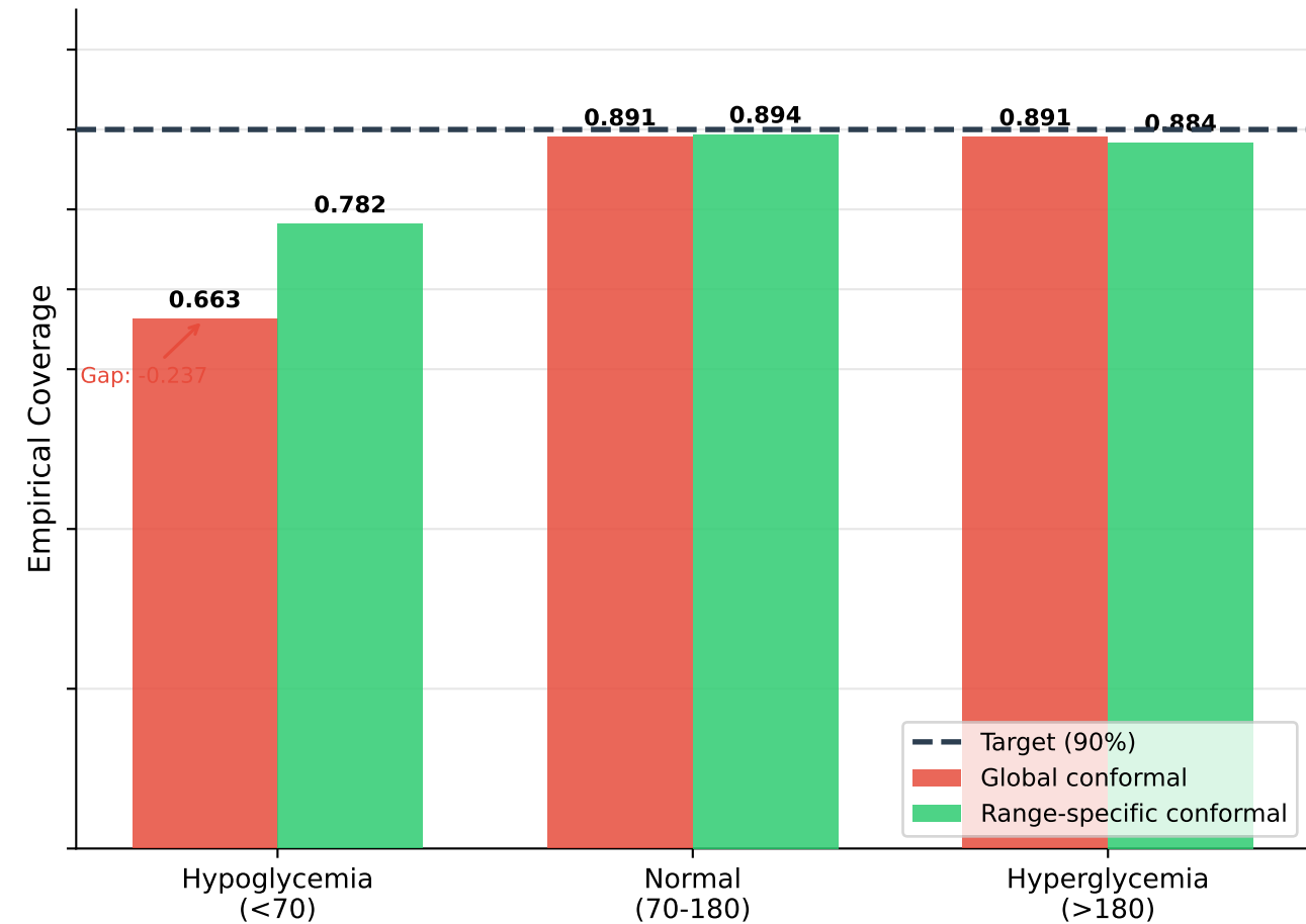
90% Prediction Interval Coverage Test Set
