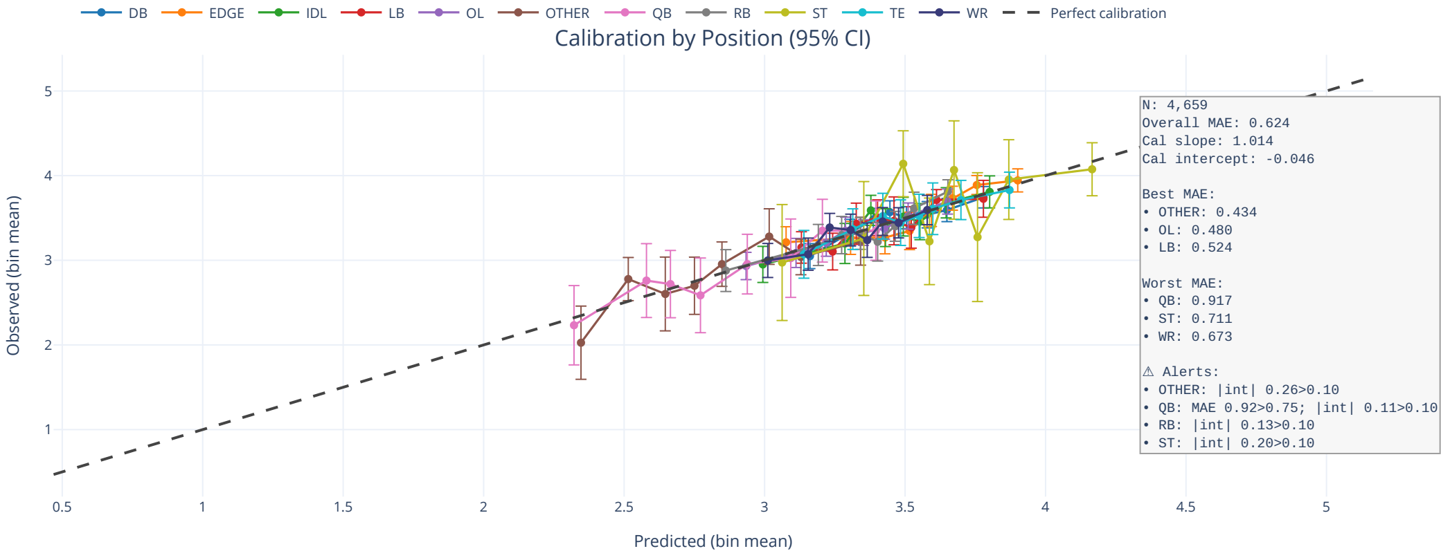
Model Diagnostics by Position
