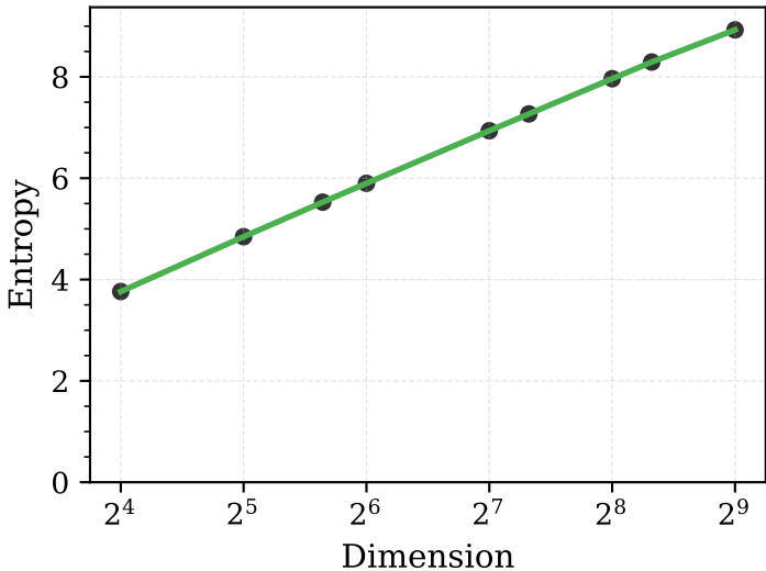
Caption Embedding Entropy
