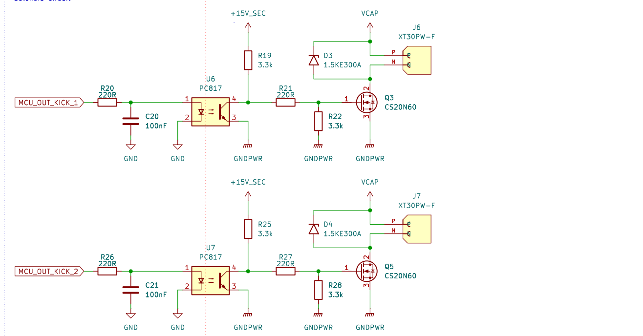
Solenoid Circuit
