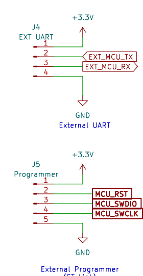
External Interfaces
