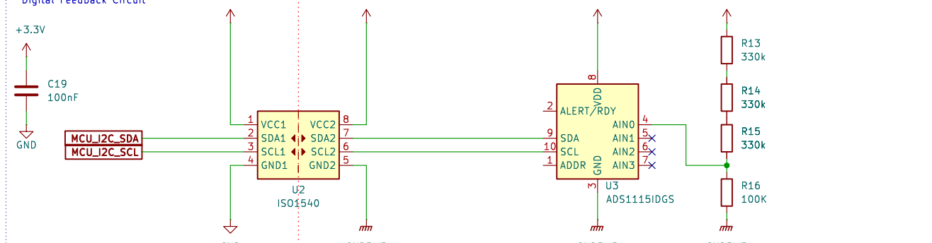
Digital Feedback Circuit
