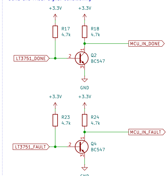
DONE and FAULT Signal Conditioning
