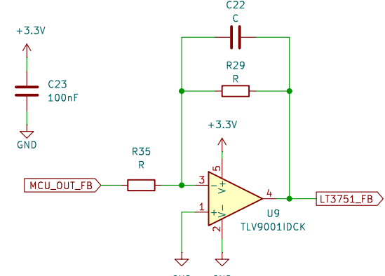
Low-Pass Active Feedback Filter
