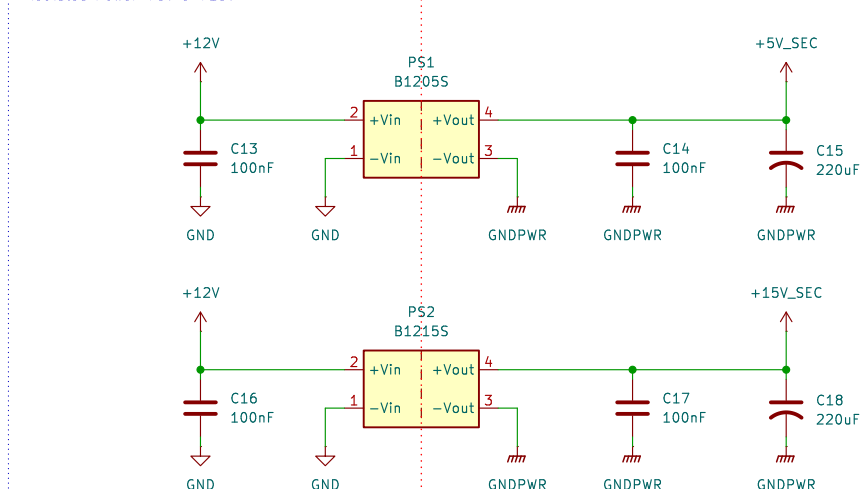
Isolated Power +5V e +15V
