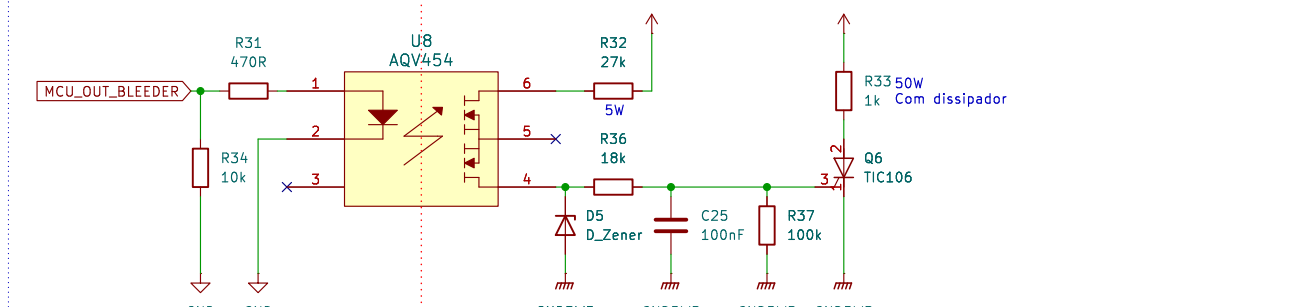
Automatic Bleeder
