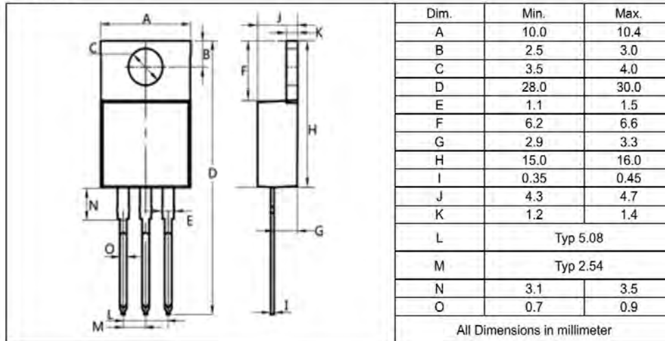
TO-220AB
