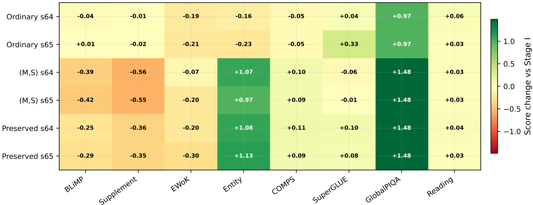
Full Endpoint x Component Delta Heatmap (vs Stage I)
