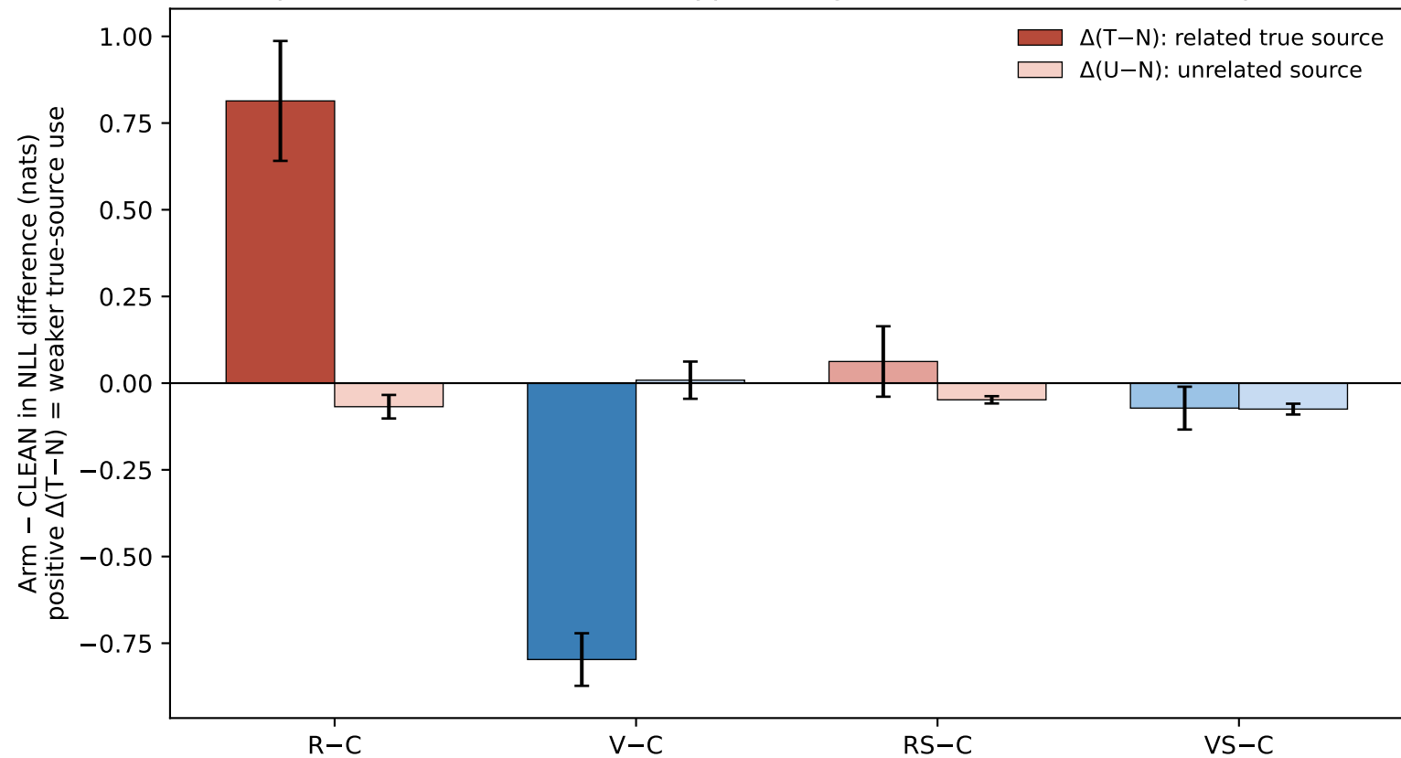
Compact rewrite T/U/N: relation type changes source-conditioned computation
