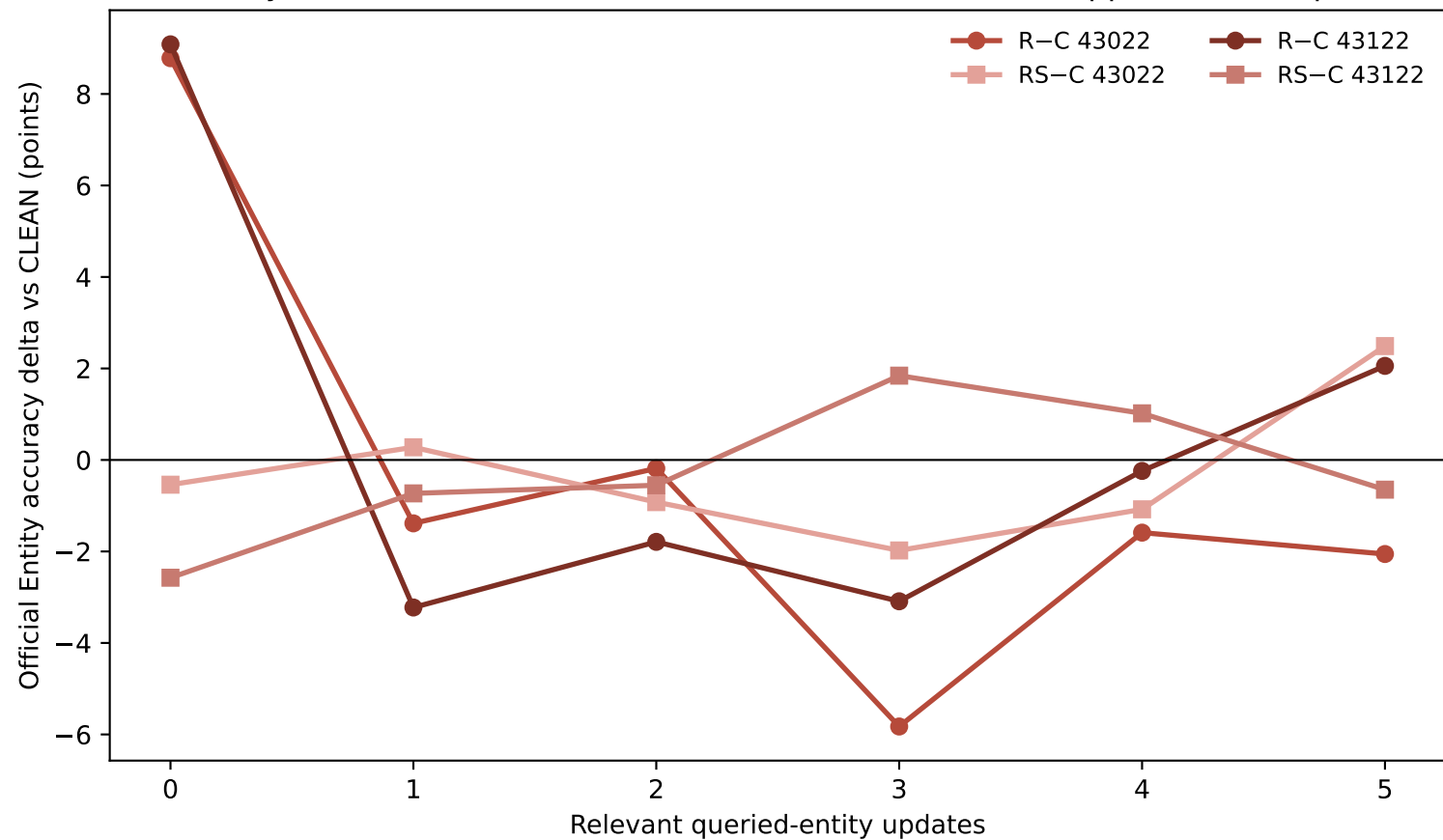
Entity behavioral face: local exact recurrence benefit disappears when split
